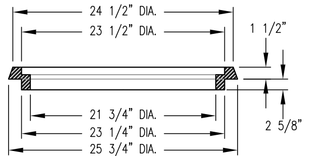
PRODUCT #1979-0180 FOR FRAME R-1924-1 1 1/2" METAL RISER
