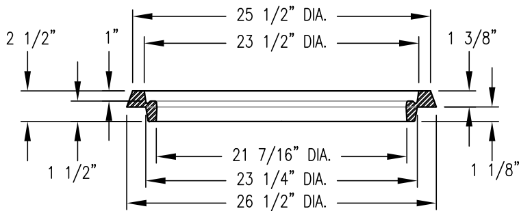
EJ NO. 2015H PRODUCT # 00201591 1 1/2" RISER RING
