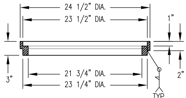
PRODUCT # NF99945222 FOR FRAME # R-1924-1 2" METAL RISER LOAD RATING: H-20 / HS-20 ASTM A36 STEEL FINISH: BLACK DIP (ASPHALT PAINT)
