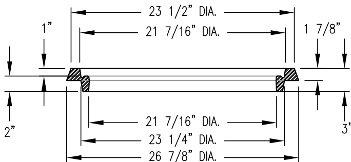
EJ NO. 2015H PRODUCT # 00201592 2" RISER RING FINISH: NOT PAINTED
